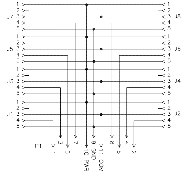
WIRING DIAGRAM
